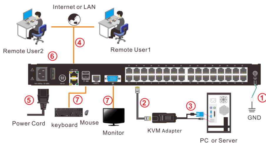
Figure 2.2 Installation diagram
