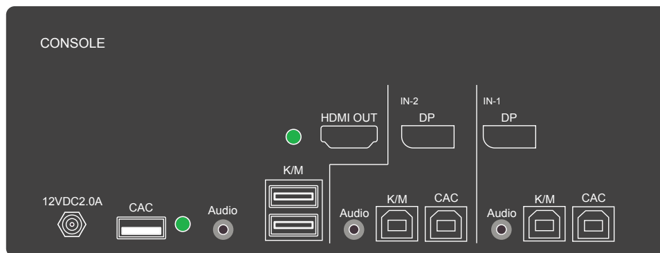
SDHN-2S-P Back
