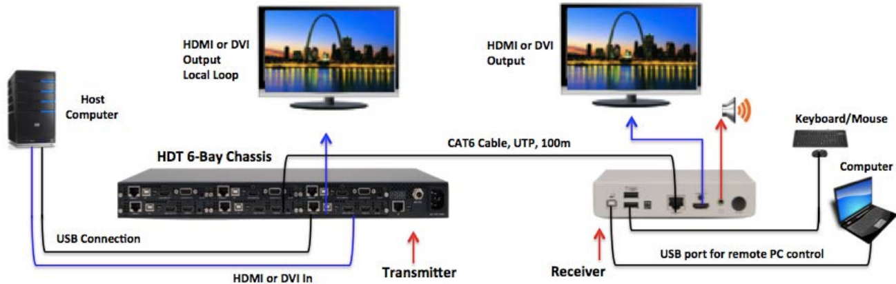
CrystalView HDT set-up when connecting to a host computer
