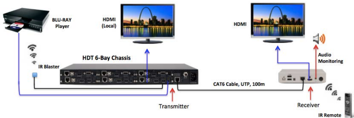
CrystalView HDT set-up when connected to a BLU-Ray video player
